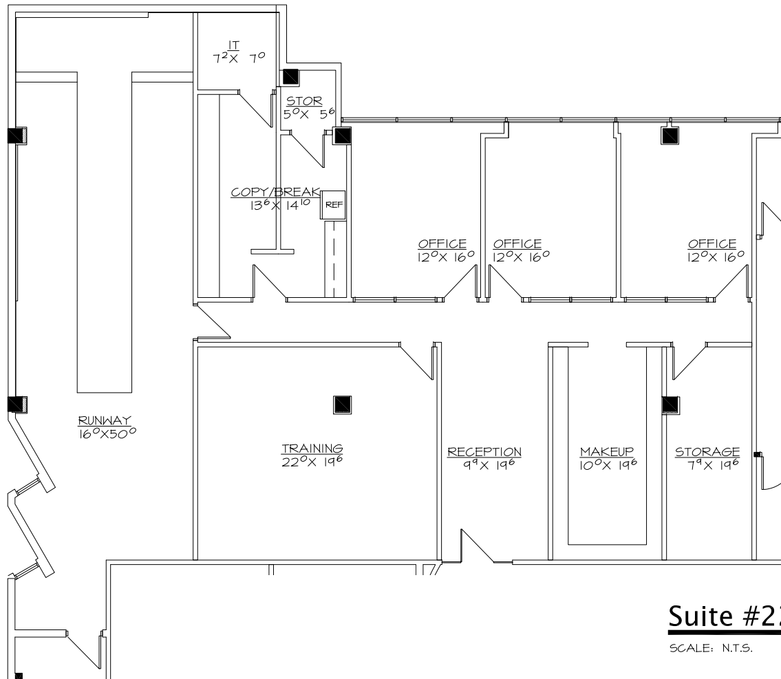
Second Floor Overall Plan
